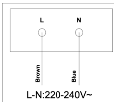
H05RR-F2G1,5*
