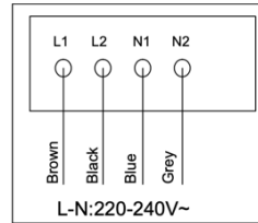
H07RN-F4G1,5*
