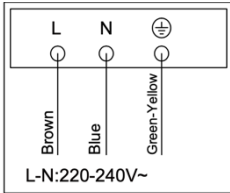
H05RR-F3G1,5*
