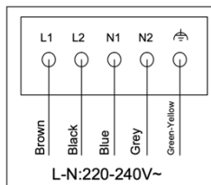
H07RN-F5G1,5*
