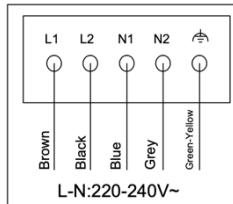
H07RN-F5G1,5*
